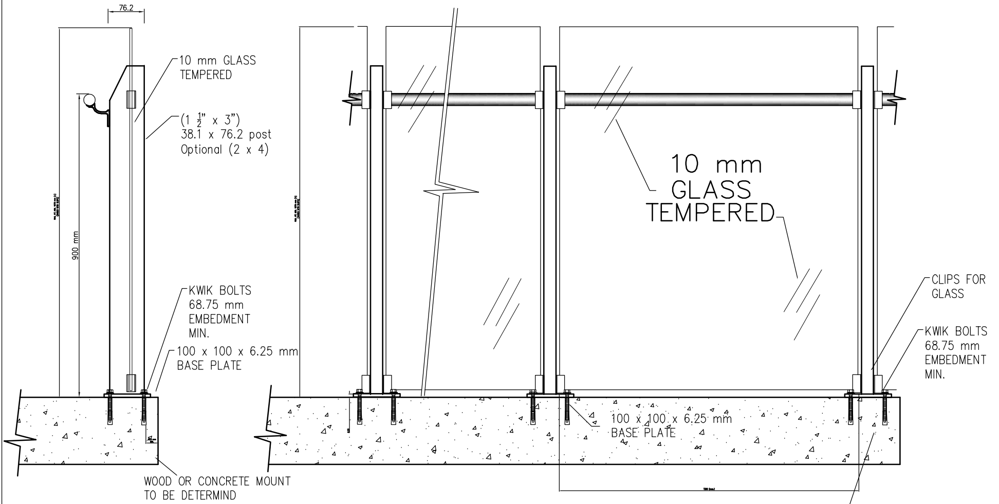
SECTION
