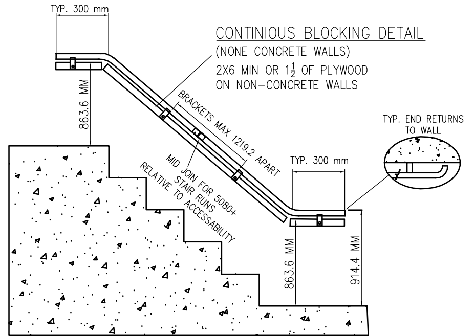
TYPICAL CORE HAND RAIL JOIN DETAIL.
