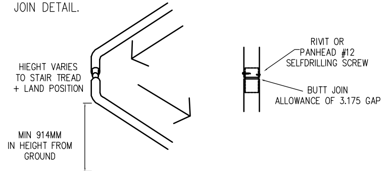
TYPICAL CORE HAND RAIL JOIN DETAIL.
