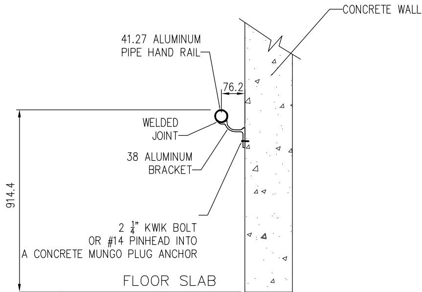
TYPICAL DETAIL OF WALL BRACKET
