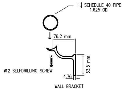
TYPICAL DETAIL OF WALL BRACKET
