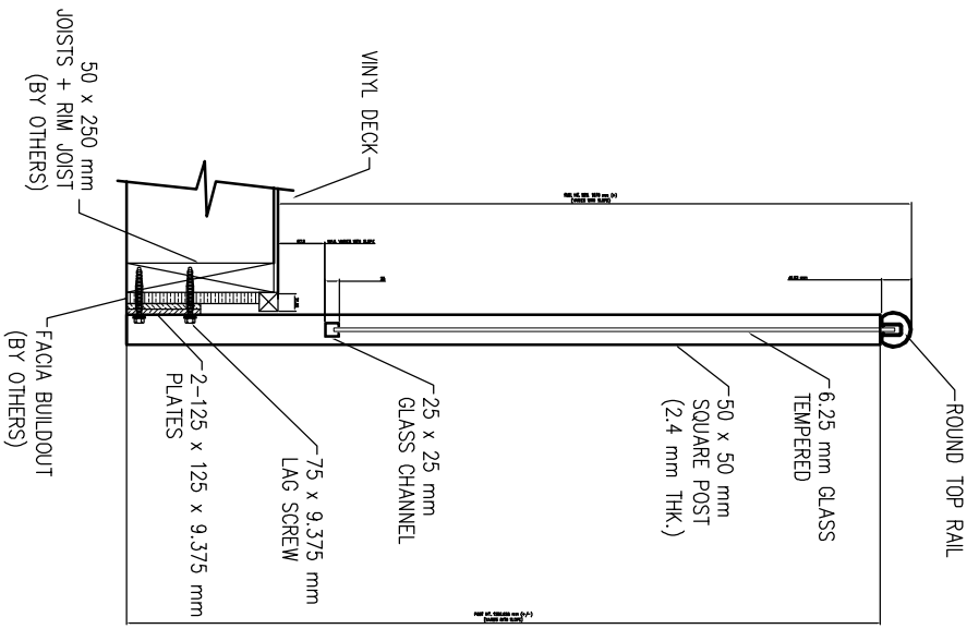
SECTION (SIDE MOUNT)
