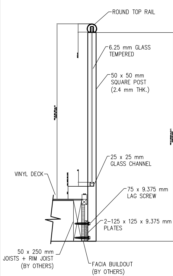
SECTION (SIDE MOUNT)
